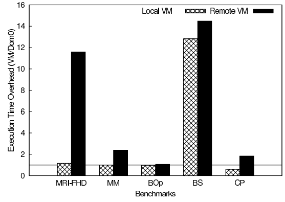
Figure 7: Application sensitivity to virtualization and network fabric overheads (Ethernet), normalized to direct execution time measurements within Dom0
