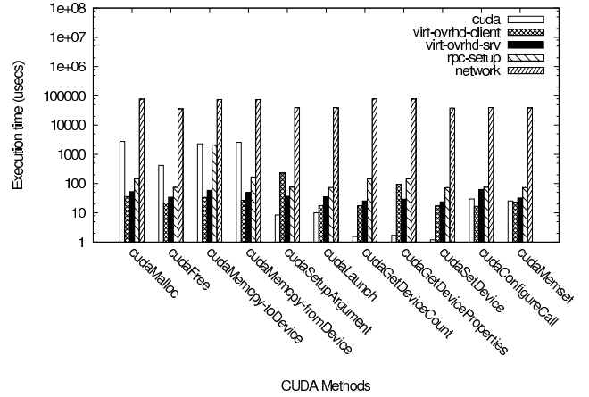
Figure 10: Profiling individual CUDA calls; breakdown of remote vGPU path (using 8 KiB data sizes for memory copies)
