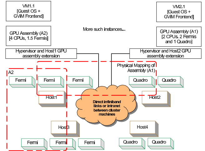
Figure 1: GPGPU assemblies spanning multiple GPGPU and CPU (implicit) nodes across a cluster for the example VMs. Partial overlap indicates partial utilization
